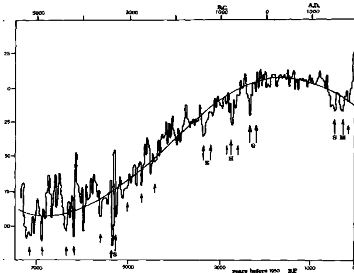
Fig. 7. ^{14}\text{C} -deviations since 5300 BC derived from analysis of dated tree rings by Damon, with smoothed curve of sinusoidal variation in the Earth's magnetic moment from Lin et al. The variations modulating the sine curve are attributed to long-term changes in solar activity. The graph after Eddy allows for the vice versa relation of cosmic ray flux with solar activity. Six grand minima (M, Maunder Minimum; S, Spoerer Minimum; G, Greek Minimum; H, Homeric Minimum; E, Egyptian Minimum; S, Sumerian Minimum) coincide with negative RDM meeting the criterion Cn3 which are marked by long arrows. All negative RDM of the category Cn2 which occurred since 5300 BC are represented by shorter arrows. The date of the youngest RDM(Cn2) is 1811.
