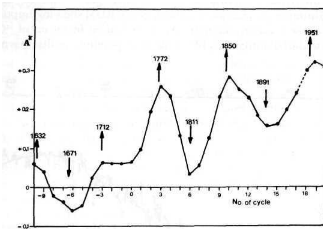
Fig. 6. Peaks and troughs in the Gleissberg cycle of sunspot activity outlined by the secularly smoothed asymmetry A^* of the 11-yr cycle. The data for cycles 18-20 are extrapolated. Synchronous positive and negative RDM are marked by arrows indicating the respective polarity. The two successive positive RDM 1712 and 1772 are properly reflected by the horizontal course of the A^* -curve after RDM 1712 appearing instead of a minimum in the plot.
