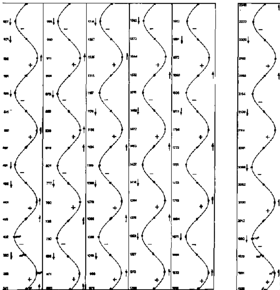
Fig. 4. Course of the 79-yr cycle from AD 341 to 2248. Positive phases ( 0 < 180^\circ ) and negative phases ( 180^\circ < 360^\circ ) are indicated by positive and negative signs. The main phases 0^\circ , 90^\circ , 180^\circ and 270^\circ coinciding with DM-potentials are represented by fat dots. Arrows pointing up or down symbolize positive or negative RDM which actualize DM-potentials on condition that the time integral of torque criterion C_n! is fulfilled. Upward arrows on the right of the wave indicate peaks, downward arrows on the left mark troughs in the secular cycle of solar variations.
