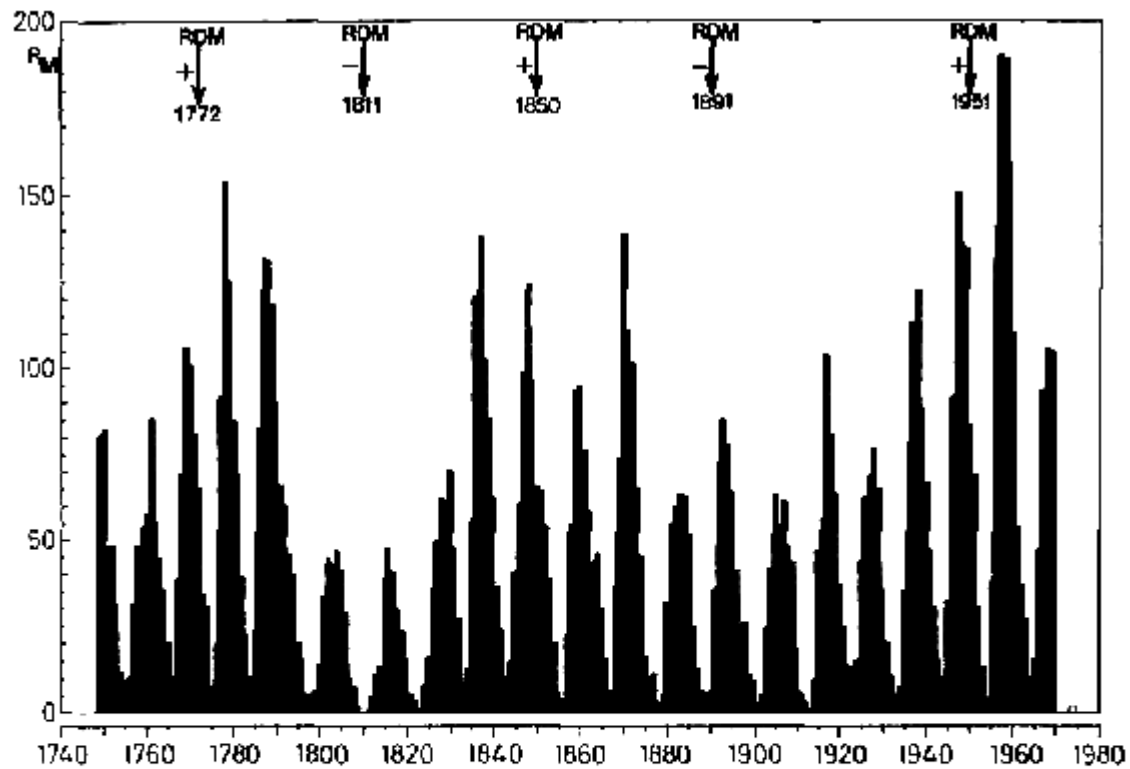
Fig. 2. Variation in the intensity of 11-yr maxima of sunspots in relation to relevant minima in the distance from the sun's center to the center of mass (RDM) showing sufficient strength of the sun's impulse of the torque to release variations in solar activity.
